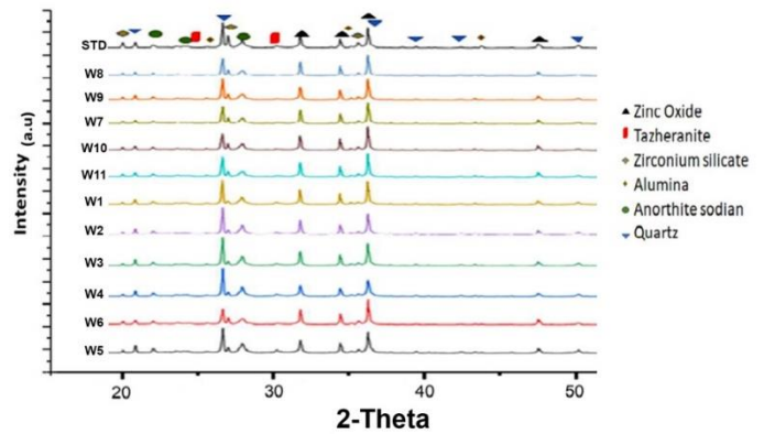
Figure 3. XRD patterns of investigated engobe samples
