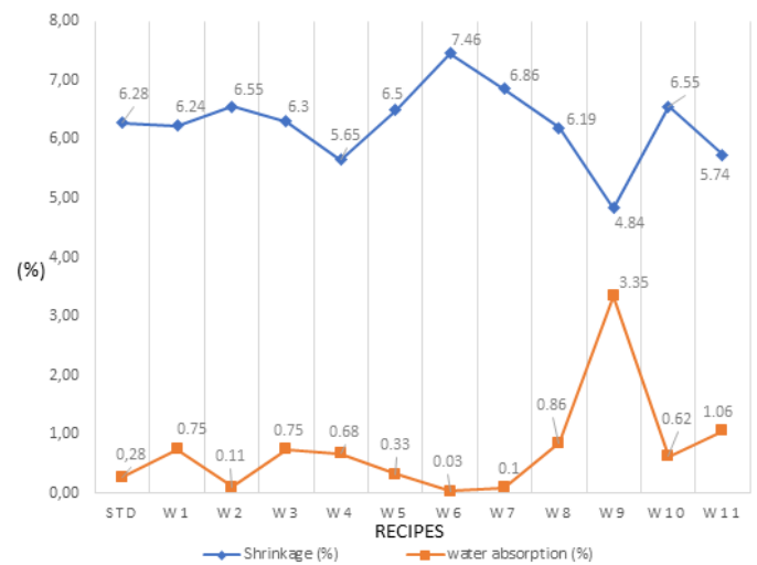
Figure 2. Shrinkage and water absorption of investigated engobe recipes
