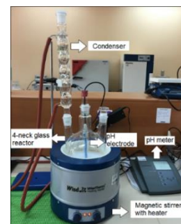
Figure 1. The experimental setup used for synthesizing the AIOOH sol via the sol-gel process.
